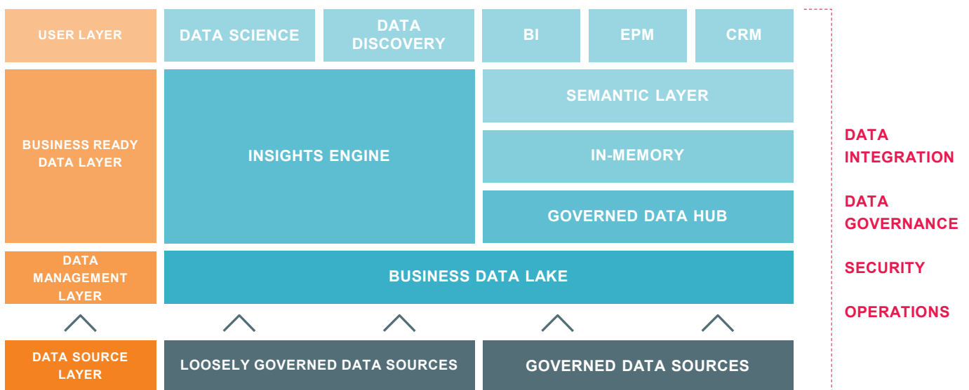
A conceptual view of MDA
